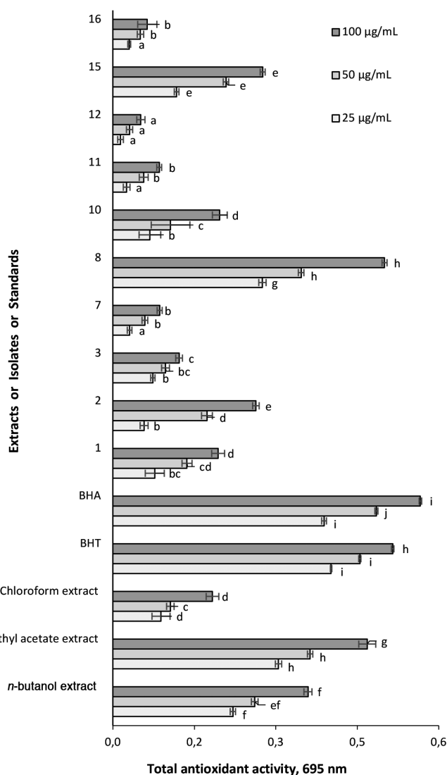
Figure 2. Total antioxidant activity of isolated and extracted samples BHA: Butylated hydroxyanisole, BHT: Butylated hydroxytoluene
